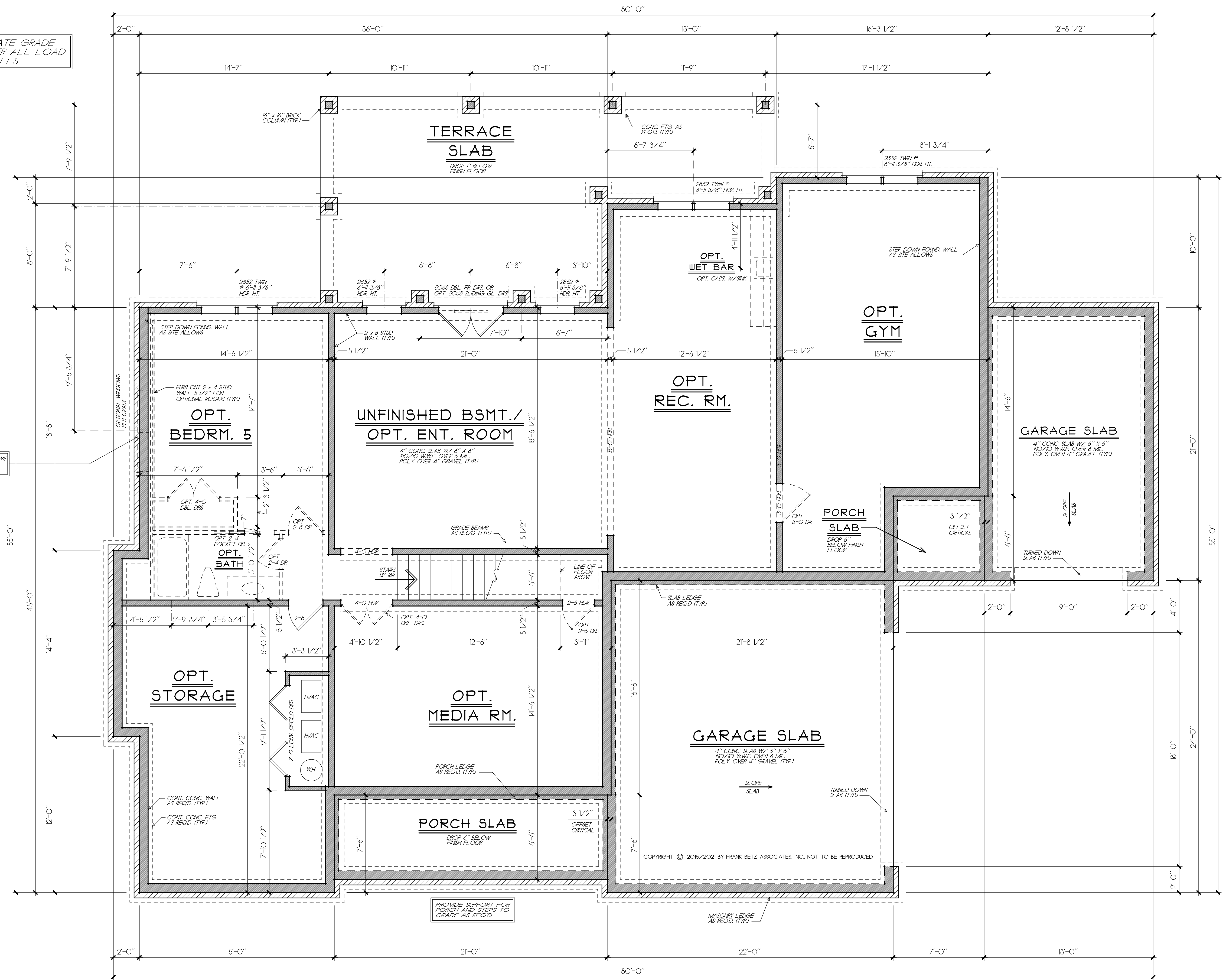
BASEMENT FOUNDATION PLAN 1/4" = 1'-0"
